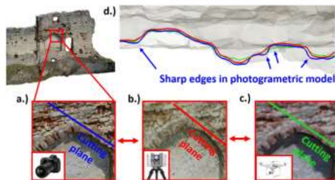
Figure 2 : Comparison between the different observation methods (a) SLR model (b) TLS model (c) UAV model (d) by using geometric cutting lines through the obtained 3D models
