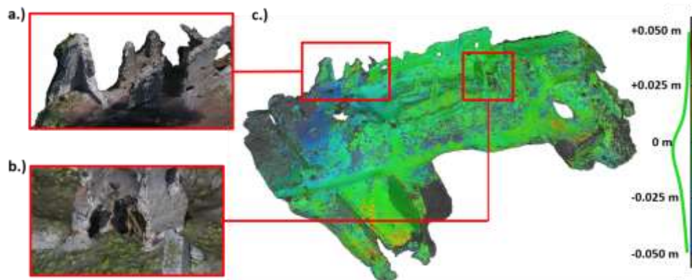
Figure 1: Cloud2Mesh comparison between laser scan (cloud) and UAV (mesh) data with detail images of (a) the northern living quarters and (b) the kitchen
